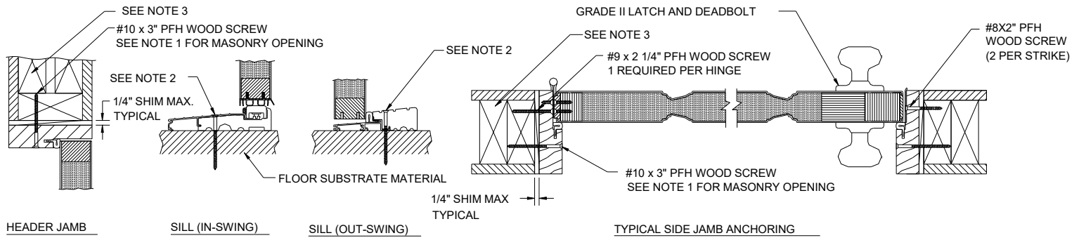
SINGLE DOOR W/ SIDELITE (BOXED)
