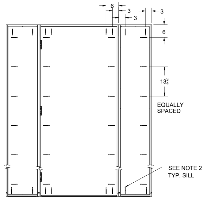
SINGLE DOOR W/ SIDELITES (BOXED)
