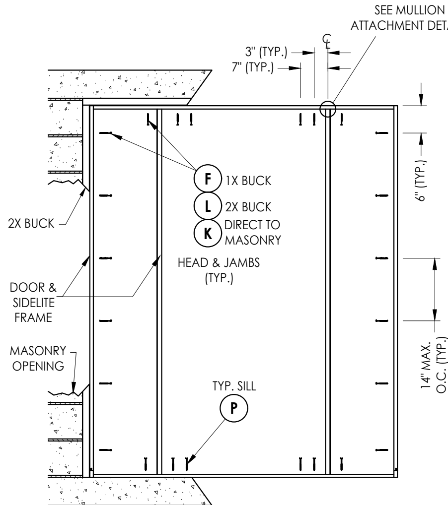
FRAME ANCHORING Masonry construction
