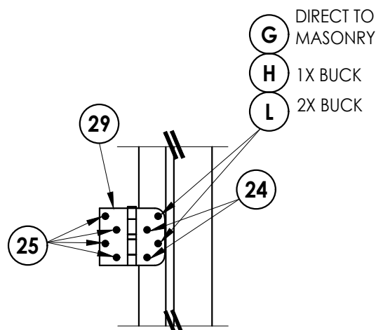
HINGE DETAIL 1
