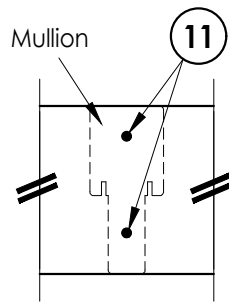
MULLION ATTACHMENT DETAILS Required at the head and sill
