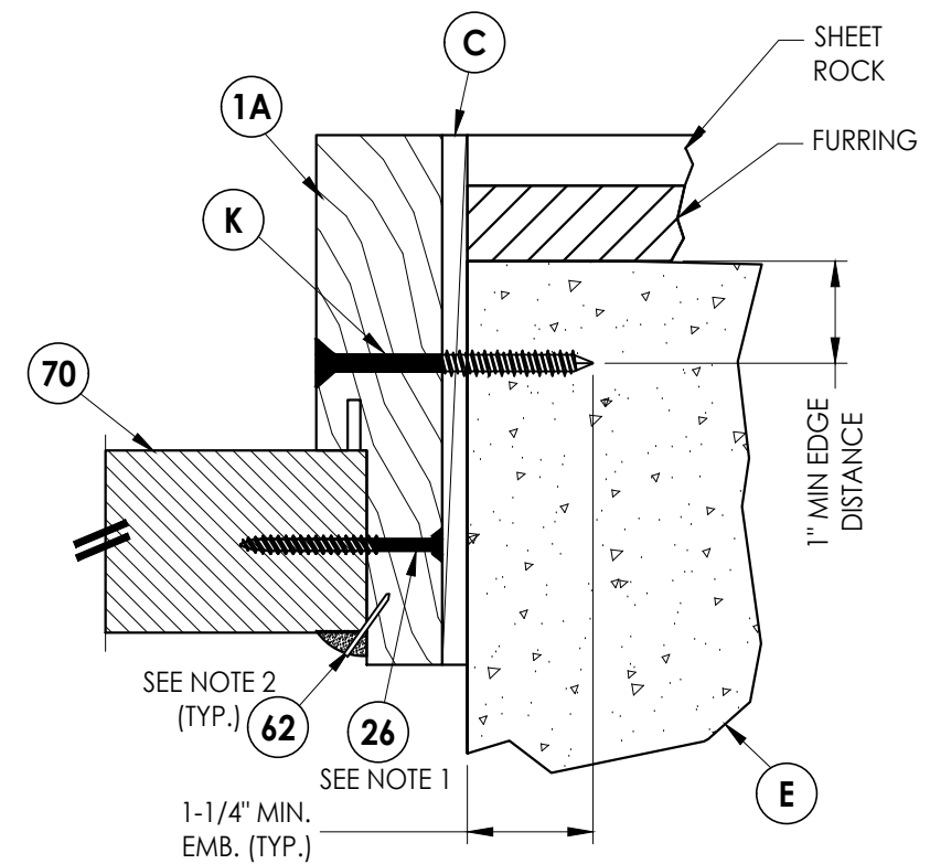
2 7 HORIZONTAL CROSS SECTION Outswing only
