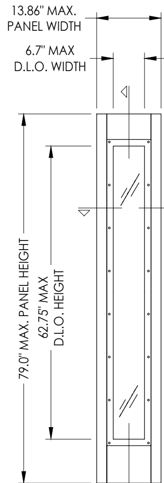
2 3 70 SIDELITE PANEL
