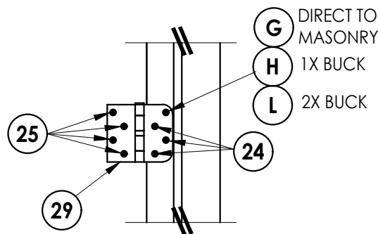
HINGE DETAIL 2
