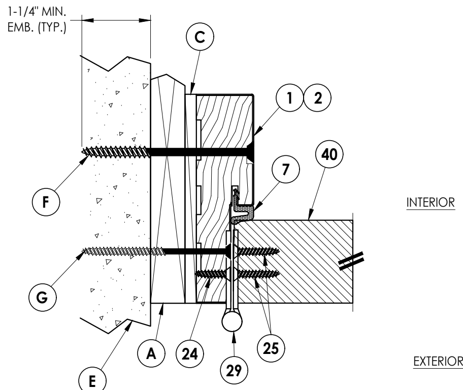
1 6 HORIZONTAL CROSS SECTION Outswing shown - Inswing also approved
