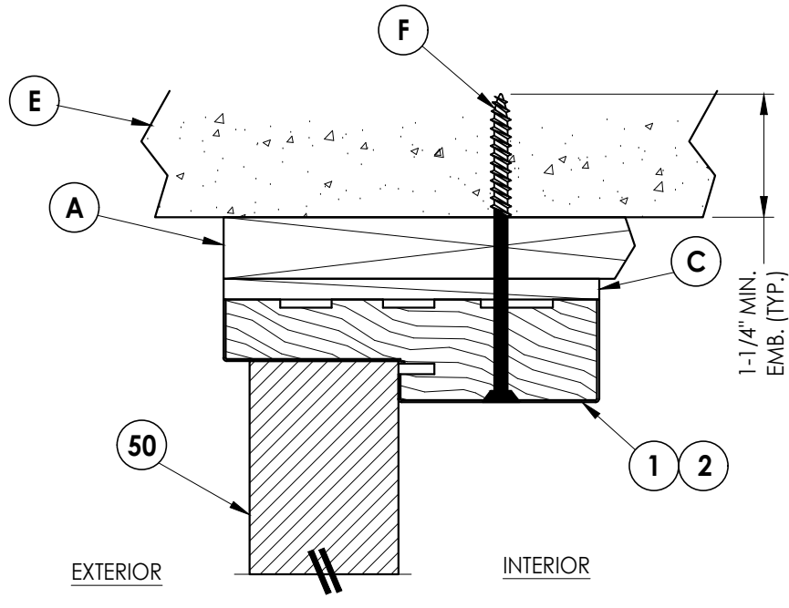
5 6 VERTICAL CROSS SECTION Outswing shown - Inswing also approved
