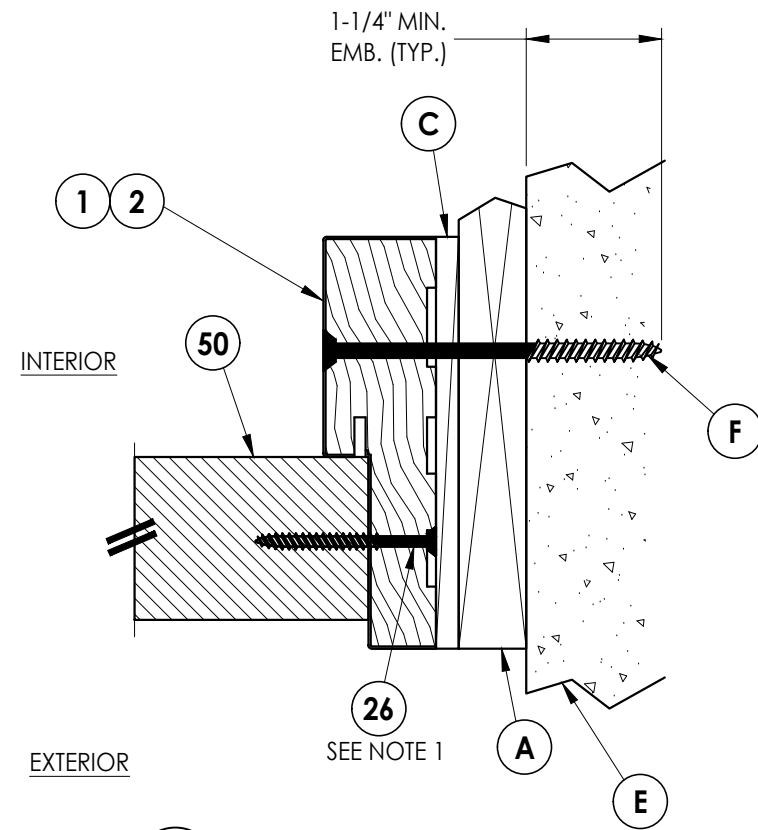
3 6 HORIZONTAL CROSS SECTION Outswing shown - Inswing also approved
