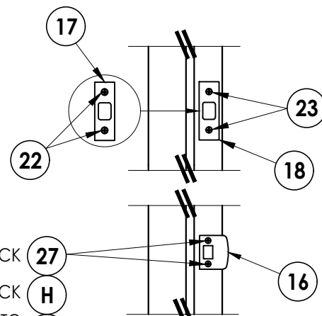
STRIKE PLATE DETAIL SCHLAGE LOCKSET
