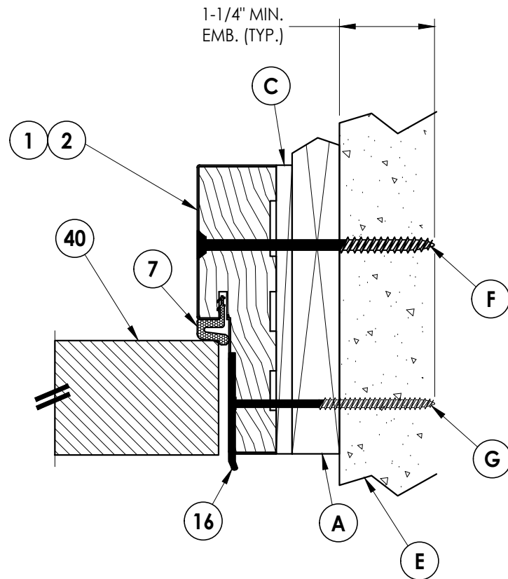
2 6 HORIZONTAL CROSS SECTION Outswing shown - Inswing also approved
