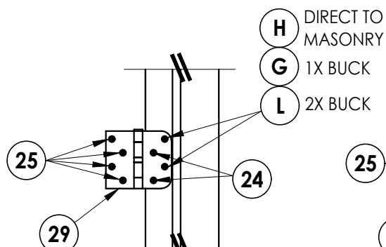
HINGE DETAIL INSWING
