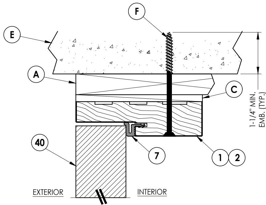
4 6 VERTICAL CROSS SECTION Outswing shown - Inswing also approved
